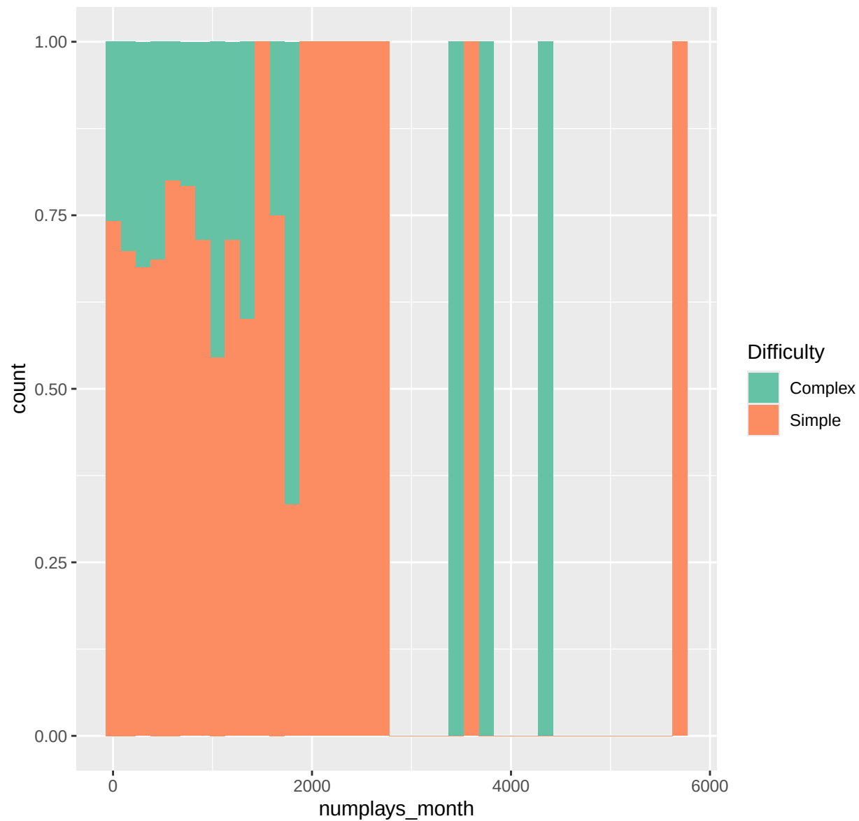
Monthly Plays by Difficulty
